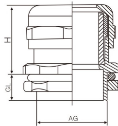
Technical diagram illustrating internal components and key dimensions including thread length (GL).
