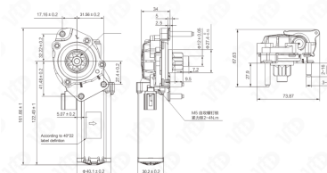
Technical diagram detailing the dimensions and mounting specifications of the VDF44 DC motor unit.
