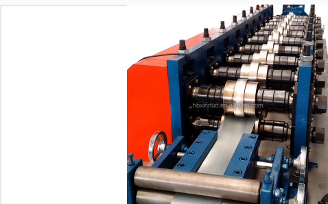
Complete production line view showing decoiler, roll forming stands, and hydraulic cutting system.
