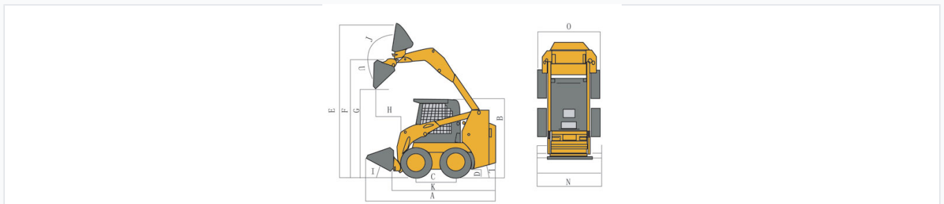
Dimensional blueprint showing the machine's footprint and key clearance points.
