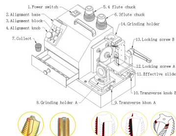
Control and adjustment interface for precise tap positioning.
