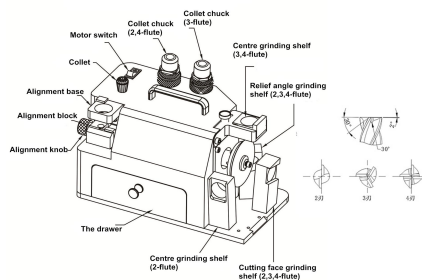
Detailed view of the grinder controls including collet chucks, alignment knobs, and various grinding shelves for 2, 3, and 4-flute tools.
