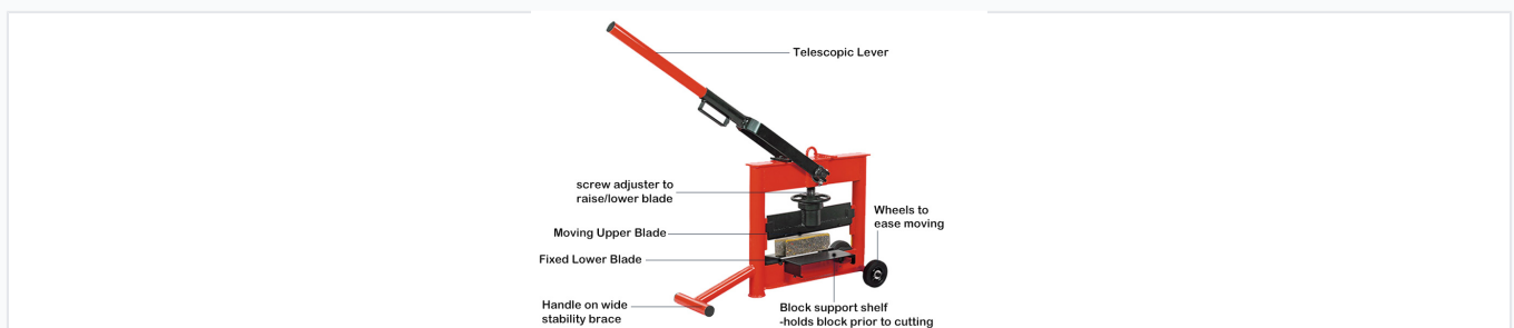
Detailed view of the splitter mechanism, featuring a telescopic lever for leverage, adjustable blade height, and a block support shelf for stability.
