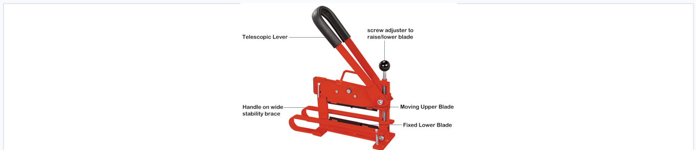
Detailed view of the functional components, including the telescopic lever, screw adjuster, and blade assembly.
