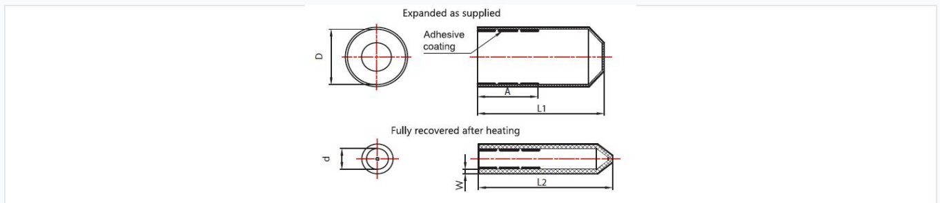
Cross-section illustration showing the adhesive coating and shrinkage process.
