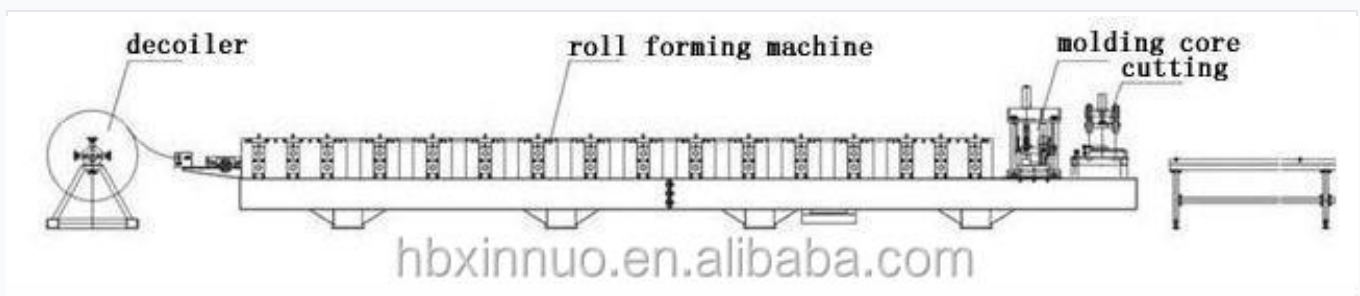
Integrated production line featuring decoiler, roll forming, and cutting sections.
