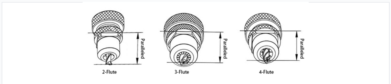
Capable of sharpening 2, 3, and 4-flute end mills with consistent results.
