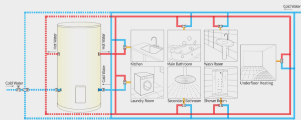
HIGH-CAPACITY MULTIPLEX WATER SUPPLY
