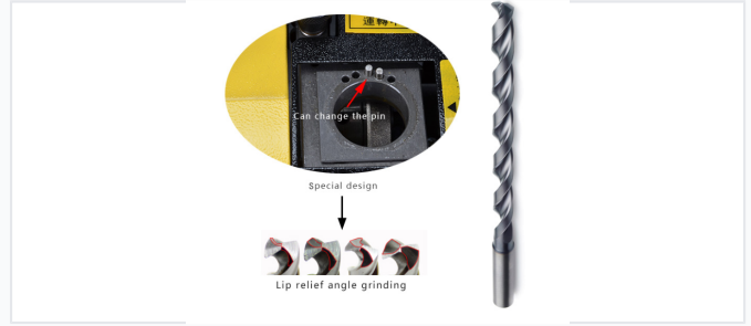
Specialized design features including lip relief angle grinding and adjustable pins.
