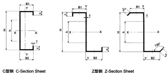
Dimensional profiles for C-section and Z-section steel sheets produced by the machine.
