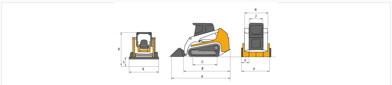
Dimensional overview showcasing wheelbase, height, and length parameters for the HT100L model.
