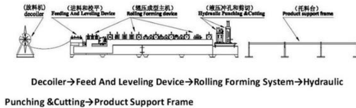
Complete production flow from decoiling to the final product support frame.
