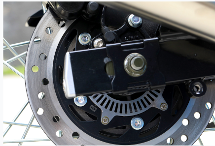
Vented disc brake rotor designed for efficient heat dissipation.
