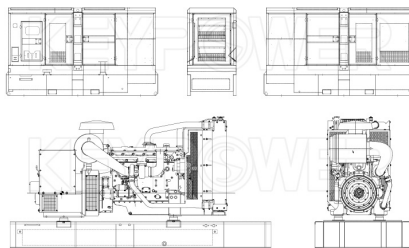
Drawing of keypower generator
