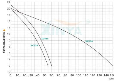
Performance characteristic curve showing Total Head (m) versus Flow Rate (L/min).
