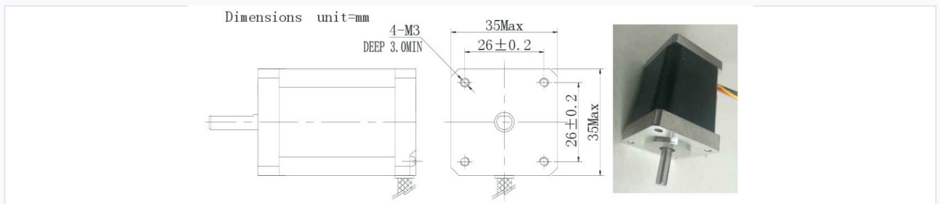
Dimensional layout and mounting specifications for the 35mm frame size.
