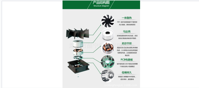
Internal view showing pure copper coils, PBT fiberglass blades, and high-precision bearings.
