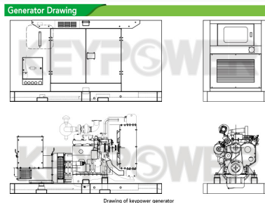
Detailed layout showing the engine, alternator, and soundproof enclosure design.
