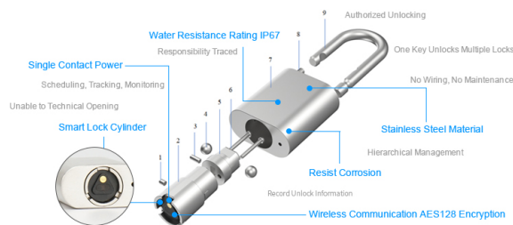
High-security features including AES128 encryption and IP67 water resistance.
