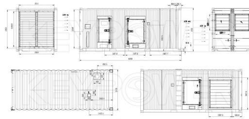
Drawing of keypower generator
