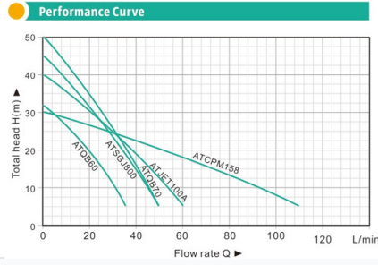
Performance curves demonstrating the relationship between head pressure and flow rate for various models.
